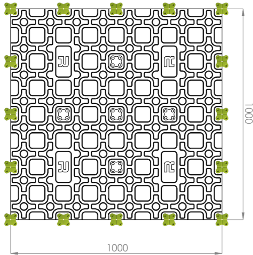
RUBTILER R-PAD BOTTOM DESIGN heavy-duty with maximum shock absorbtion and anti-fatigue properties
